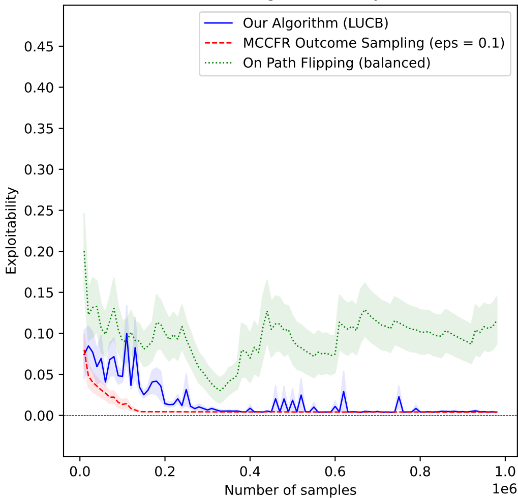
RBT, Best Algorithms, Player x
